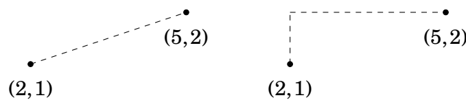
Euclidean distance
